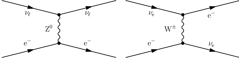
Figure 2.5.: NC (left) and CC (right) neutrino electron scattering.
