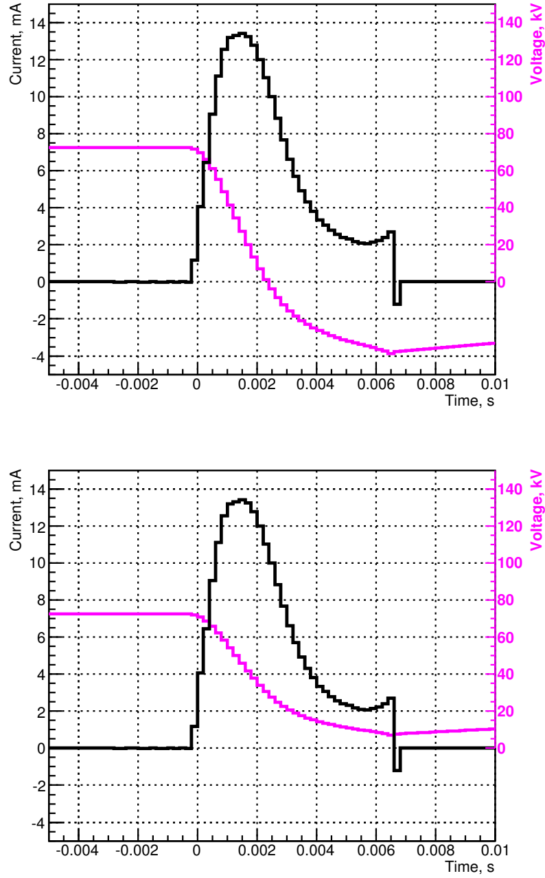
Figure 4.5.: Measured current through the gap (black) and voltage across the gap (magenta) for a typical breakdown at 6.0 mm distance between a 4 cm diameter cathode and the anode plate. The top plot shows the voltage obtained using the measured values of the protection resistor and the gap capacitance while the bottom plot uses the tuned values.
