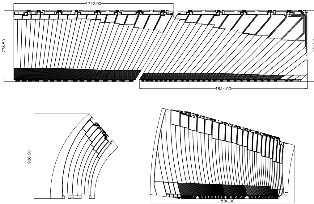
Figure 5.3: Layout of the signal layer for the four different types of electrodes before folding. The two top electrodes are for the barrel and the two bottom electrodes are for the end-cap inner (left) and outer (right) wheels. Dimensions are in millimetres. The drawings are all at the same scale. The two or three different layers in depth are clearly visible.
