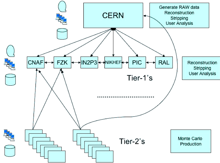
Figure 9.2: Schematic of the LHCb Computing Model.
